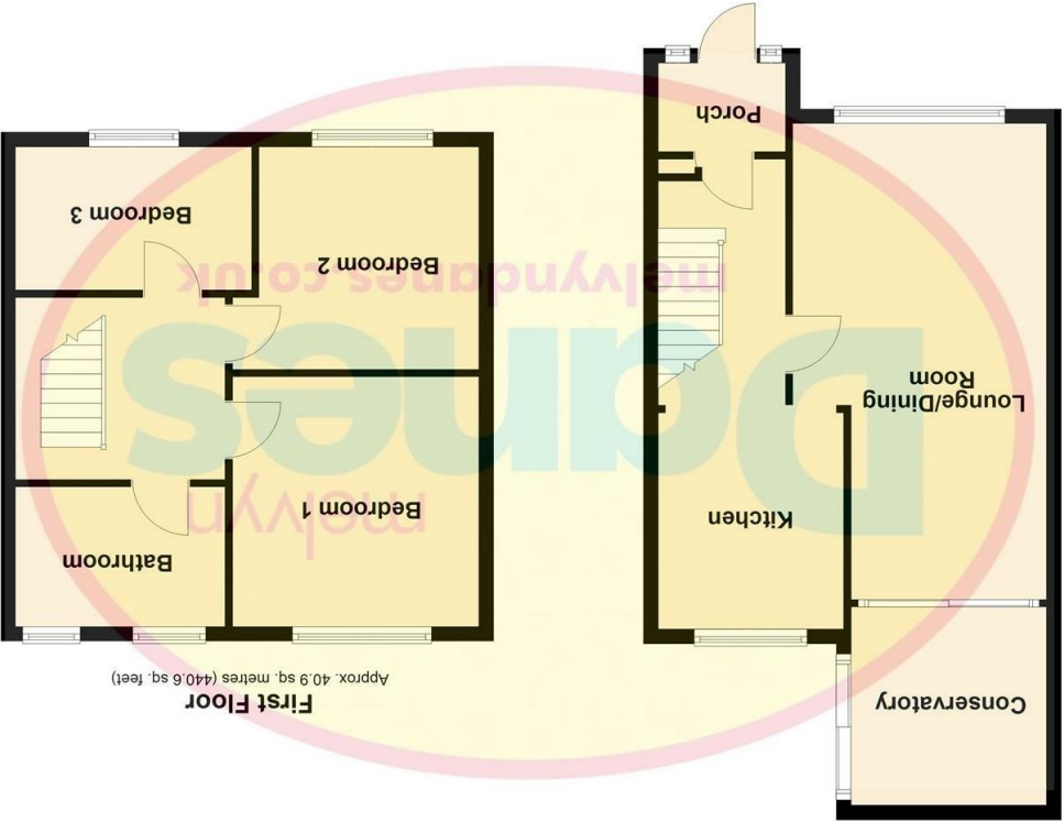
Ground Floor Approx. 49.7 sq. metres (534.6 sq. feet)
